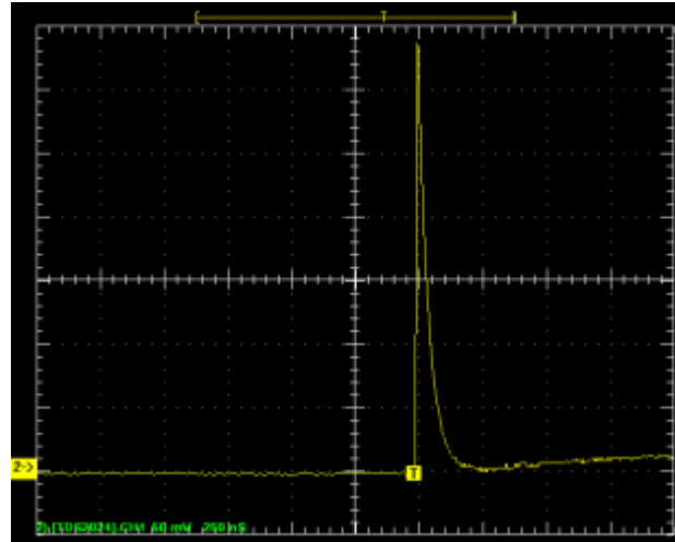
FTA001 Amplifier output shown inverted has 1ns rise time pulse
